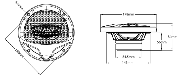
Pair of 6.6" 4-way quadaxial speakers with PP injected cone including mounting hardware
