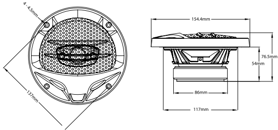
Pair of 5.4" 4-way quadaxial speakers with PP injected cone including mounting hardware
